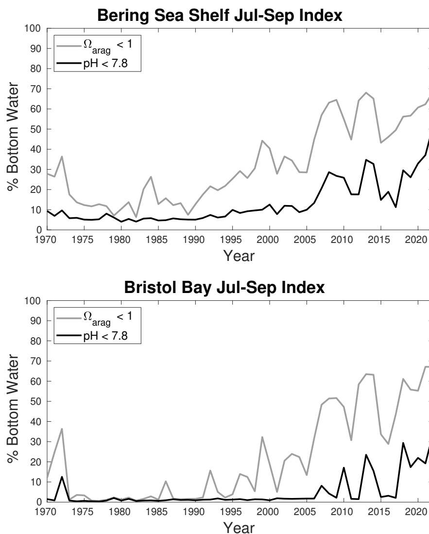
610 Figure 15: Timeseries plots of an OA indicator calculated as the spatial extent (i.e. percent of total area) of bottom waters with a July-September \Omega_{\text{arag}} < 1 (grey line) and pH < 7.8 (black line). The total spatial are is the entire Bering Sea shelf for the top plot and Bristol Bay for the bottom plot.
