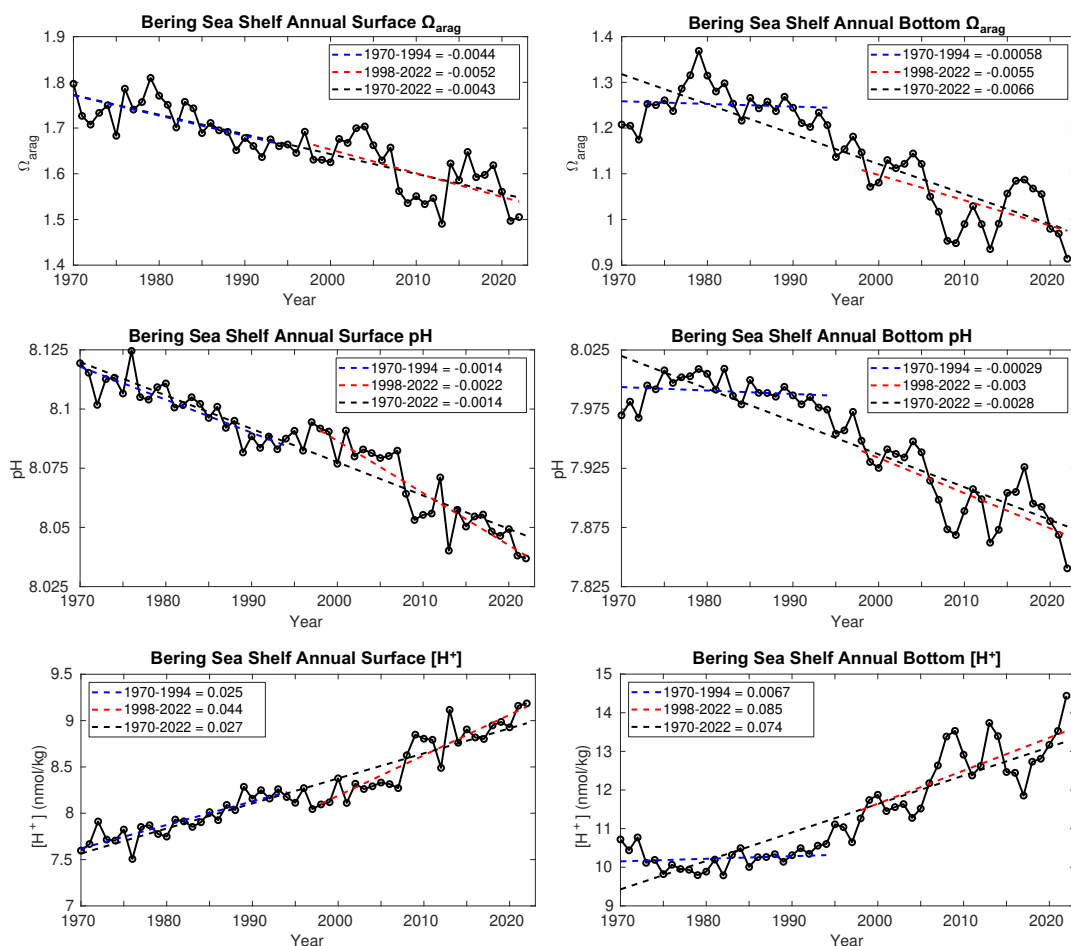
Figure 6: Timeseries plots of model annual average surface (left) and bottom (right) \Omega_{\text{arag}} (top), pH (middle), and [\text{H}^+] bottom averaged over the Bering Sea shelf region. Also shown are the linear trend values over three different timeframes.
