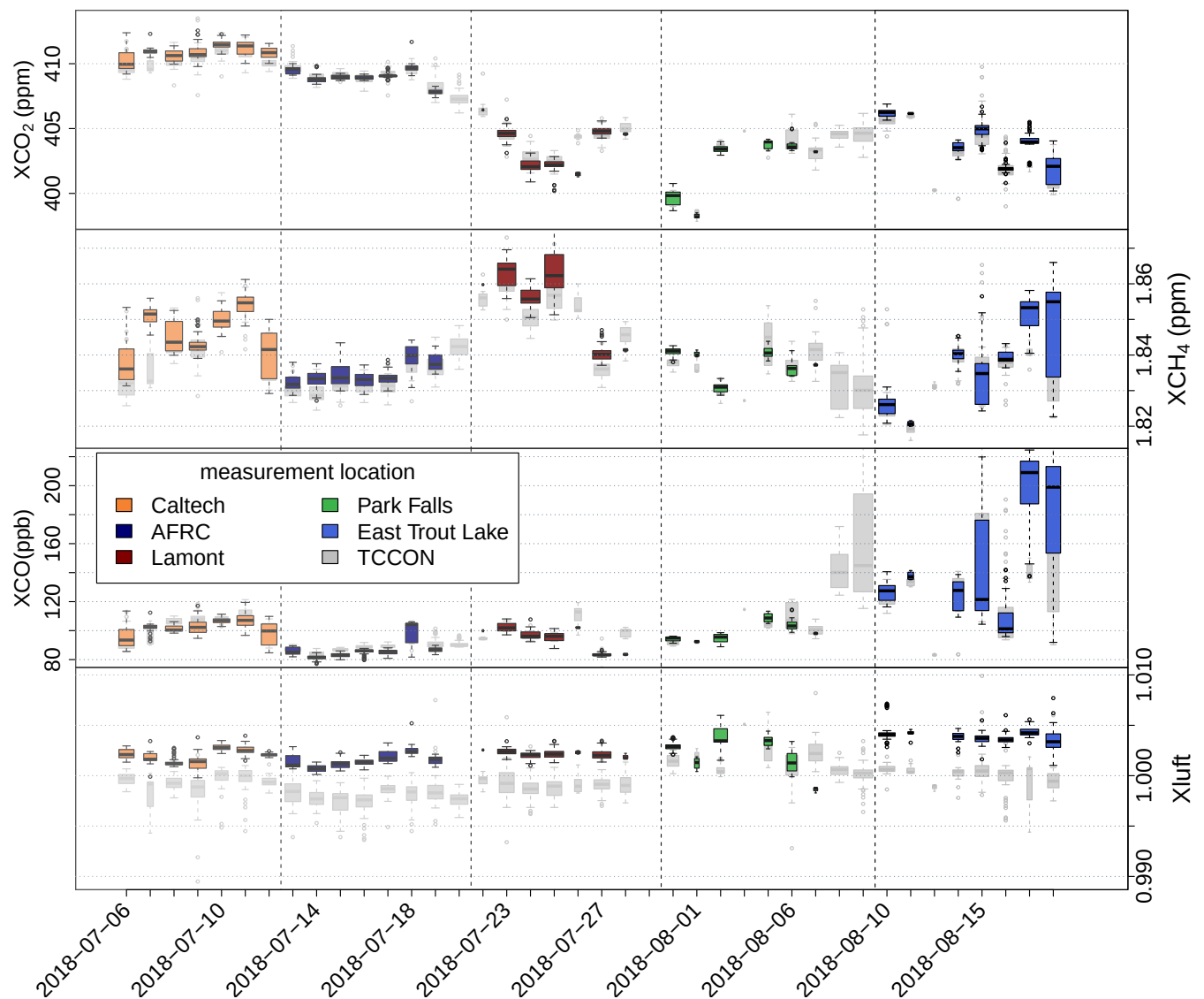
Figure 8. Timeseries of EM27/SUN (“tb”) retrieved \text{XCO}_2 , \text{XCH}_4 , \text{XCO} and \text{Xlft} in colour and co-located TCCON in transparent grey during the summer 2018 campaign (GGG2020). Different sites are highlighted by a different colour. Vertical dashed lines represent the dates in which the instruments were moved to the next TCCON station. The boxplot width is proportional to the number of observations collected in each day. The line inside each box represents the median value for each day and the bars show the daily range excluding the outliers. Outliers are depicted as dots.
