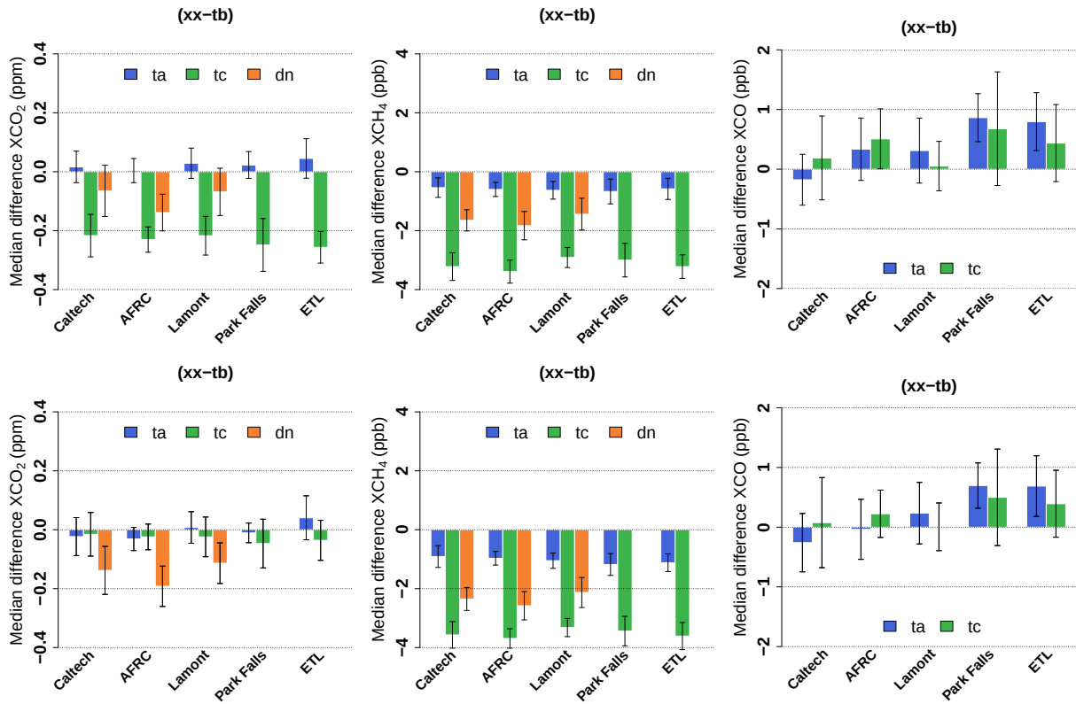
Figure 6. These figures show the median differences between the 10-minute averaged EM27/SUN \text{XCO}_2 (in ppm), \text{XCH}_4 and \text{XCO} (both in ppb) from coincident EM27/SUN measurements collected throughout the 2018 field campaign at each TCCON site before applying the instrument-to-instrument bias correction. The colour bars show the median biases of each EM27/SUN (“ta”, “tc” and “dn”) relative to the “tb” EM27/SUN instrument at each stop during the field trip. Top panel shows GGG2014 and the bottom panel GGG2020 results respectively. The error bars on each colour bar represent the median absolute deviation in the 10-minute averaged biases.
