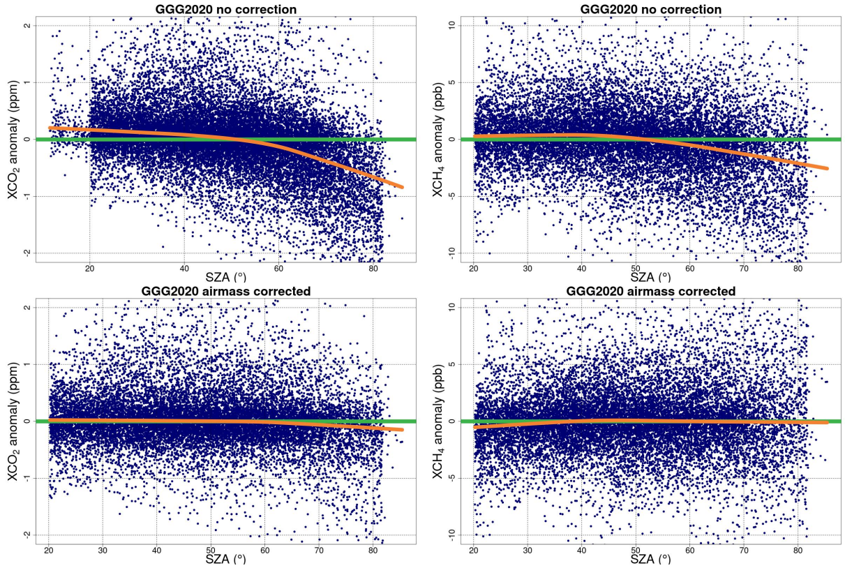
Figure 5. Daily \text{XCO}_2 and \text{XCH}_4 anomalies of the EM27/SUN (“ta”) measured in Toronto from 2017 to 2021 and during the road trip in 2018 vs. solar zenith angle using GGG2020: top panel no ADCF applied, and the bottom panel the derived ADCF for the EM27/SUNs are applied. The orange line is the Lowess curve fit. The green horizontal line is the y=0 line.
